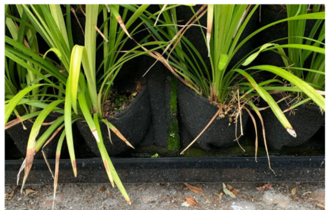
Fig. 1. Photo of the Fytotextile living wall system.
